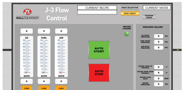
Touchscreen control
